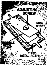
Trimmer capacitor.
